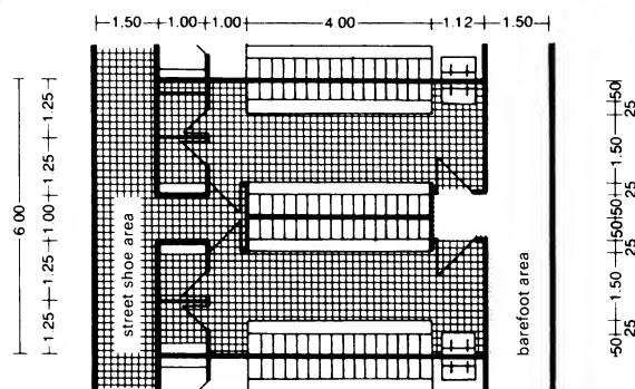
⑤ Changing area, mixed type
